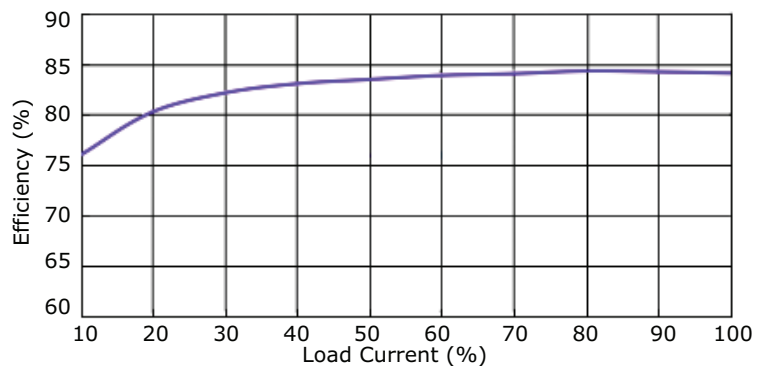
AE40-EW-S15-DIN Efficiency Curve Efficiency vs. Load Current
